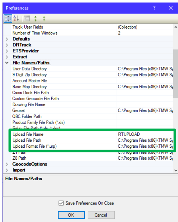
Figure 169—Upload File Name/Path
